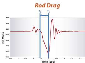
Coil Impedance
